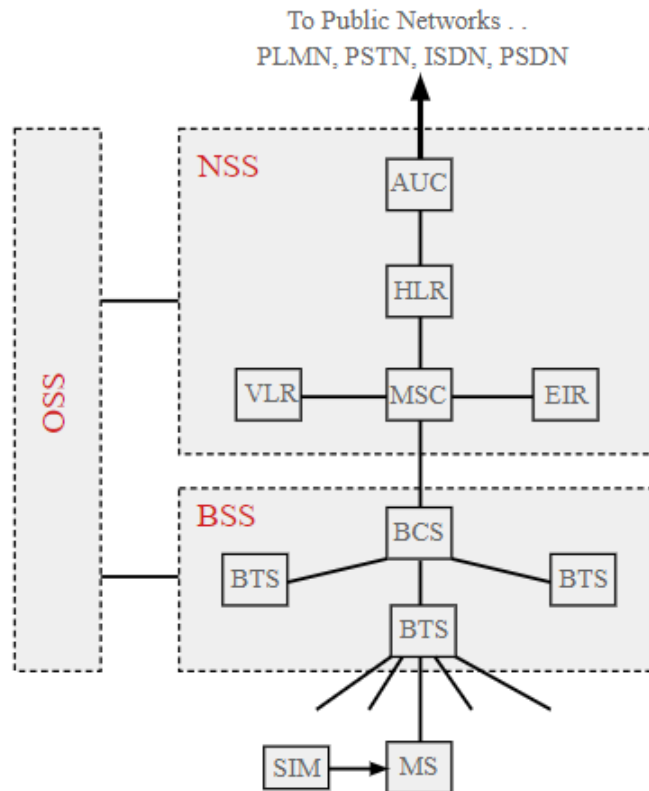
Figure 2.12: GSM Architecture
