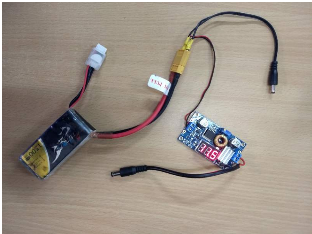
Figure 3.4: Power Supply SetUp.
