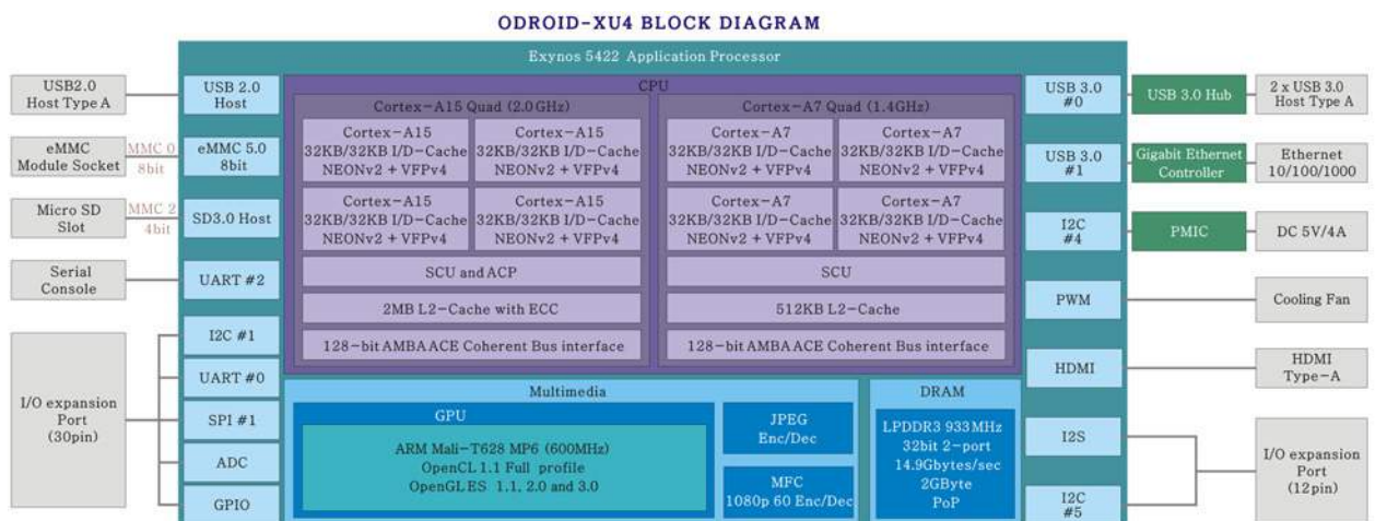
Figure 3.3: Odroid-XU4 Block Diagram.
