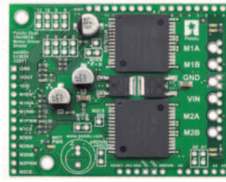
Figure 4.1: Pololu Dual VNH5019 Motor driver Board
